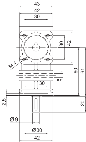
R9
